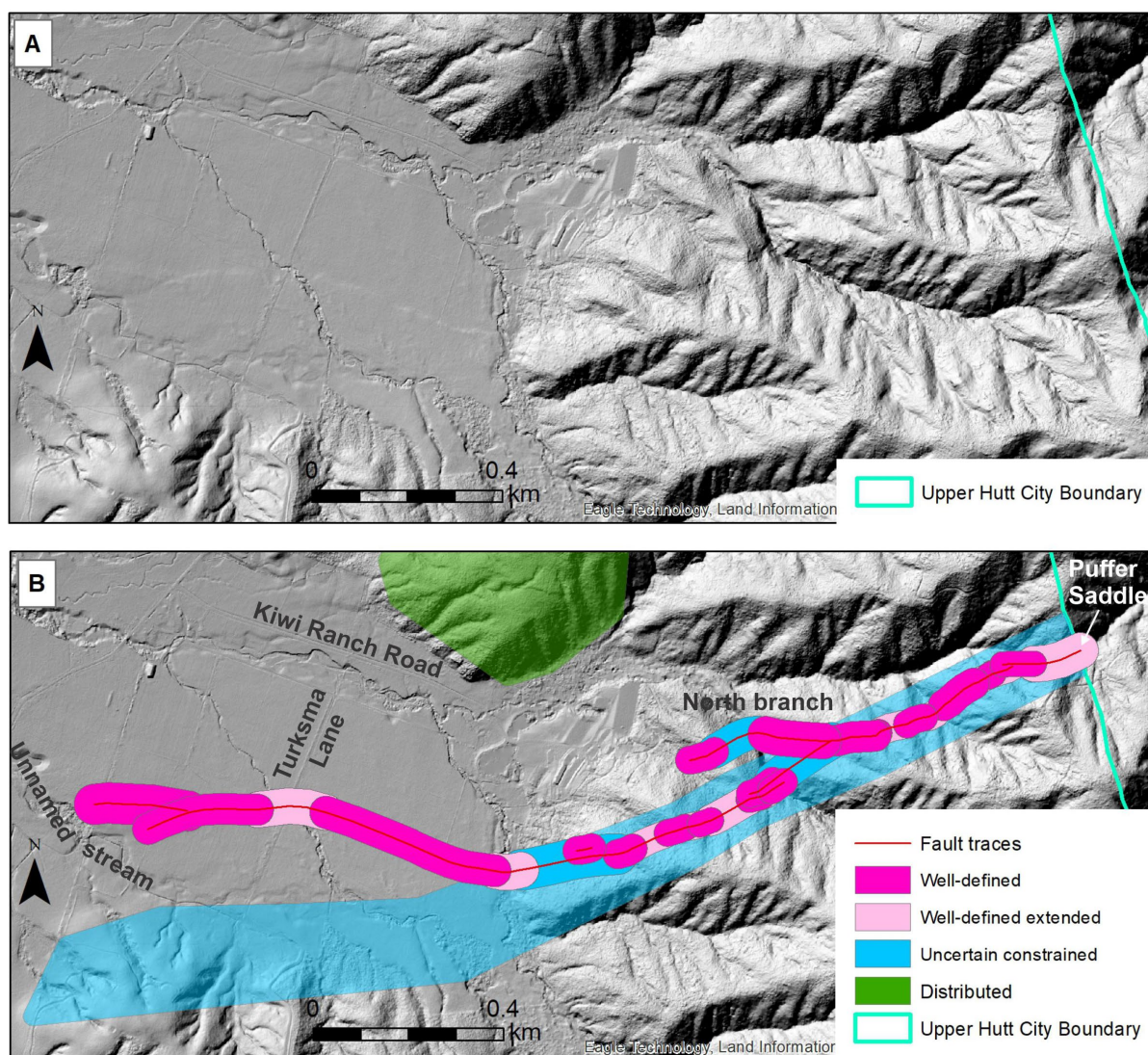
Figure 3.1 Turksma Lane strand of the Wellington Fault. (A) LiDAR hillshade map. (B) Active faults (red lines) and revised FAZs (solid coloured polygons of magenta, pink and blue) overlain on the previous (Van Dissen et al. 2005) FAZs (transparent coloured polygons of green and light blue).
