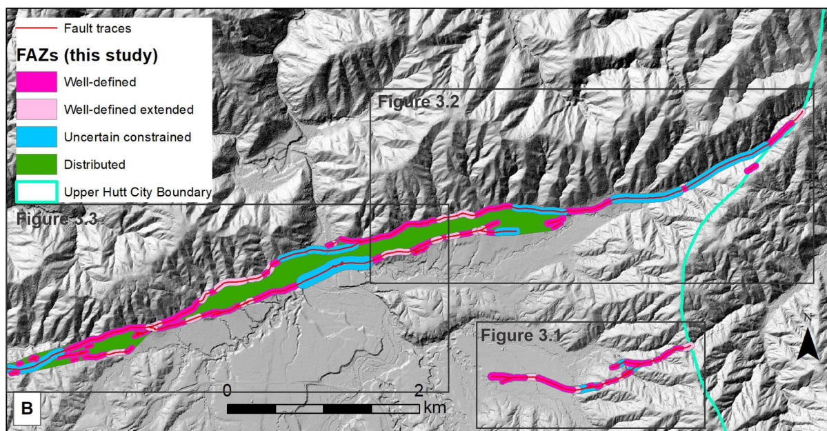
Figure 2.1 The Wellington Fault east of Te Marua Water Treatment Plant in Upper Hutt City. (A) Previous mapping in Upper Hutt City by Van Dissen et al. (2005) and in South Wairarapa District by Litchfield et al. (in press). (B) Active fault traces (red lines) and FAZs (shaded polygons of magenta, pink, light blue and green) mapped in this study. The background map in (B) is the 1 m LiDAR hillshade model.
