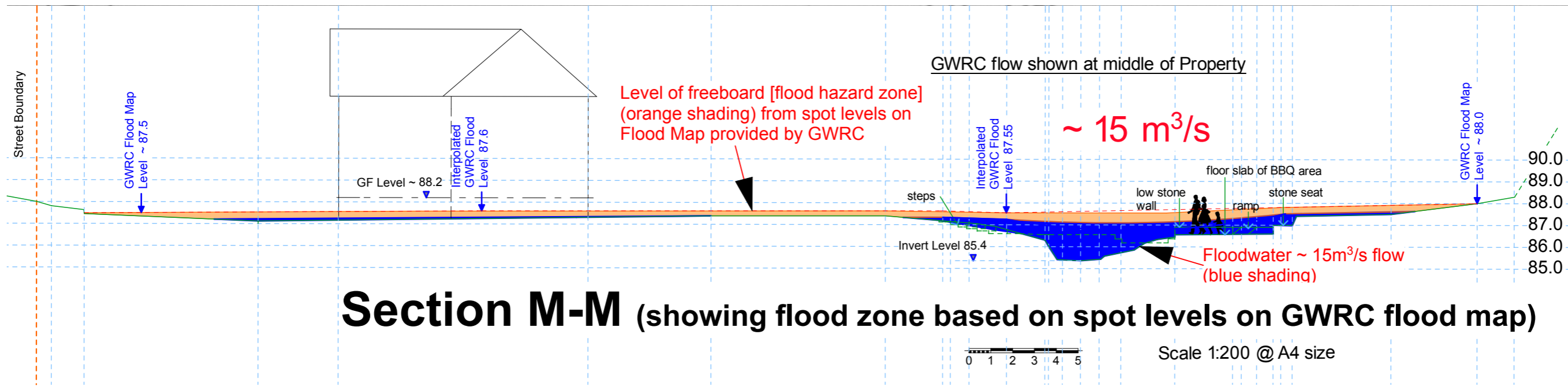
Section MM_Cross-Section through middle of GWRC Flood Map 1:200
